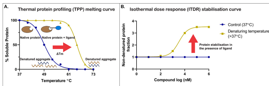
Fig. 2. A. Example melting curve for thermal protein profiling (TPP) CETSA. \Delta T_m represents the increased thermal melting temperature of the target protein in the presence of the ligand. B. Example stabilisation curve for an isothermal dose response (ITDR) CETSA. Red arrow represents the increased stability of the target protein in the presence of increasing drug concentrations following a heat challenge. (For interpretation of the references to colour in this figure legend, the reader is referred to the Web version of this article.)
