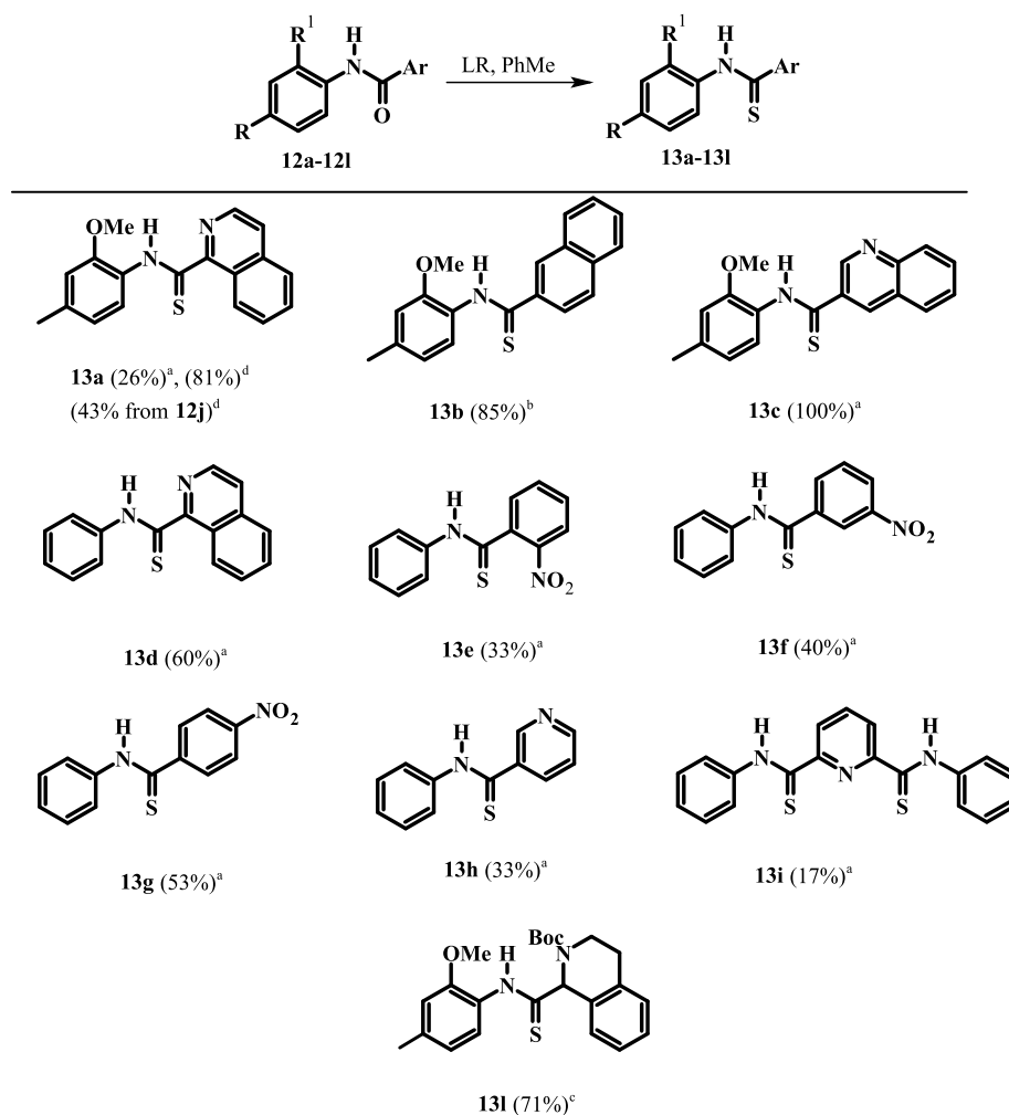
Scheme 3. Thionation of amides 12a-l using LR. a 3 mol. equiv. LR, reflux, PhMe, 24 h; b 0.6 mol. equiv. LR, reflux, PhMe, 24 h; c 1.2 mol. equiv. LR, reflux, PhMe, 24 h; d 0.6-1 mol. equiv. LR, MW, PhMe, 0.5 h.
