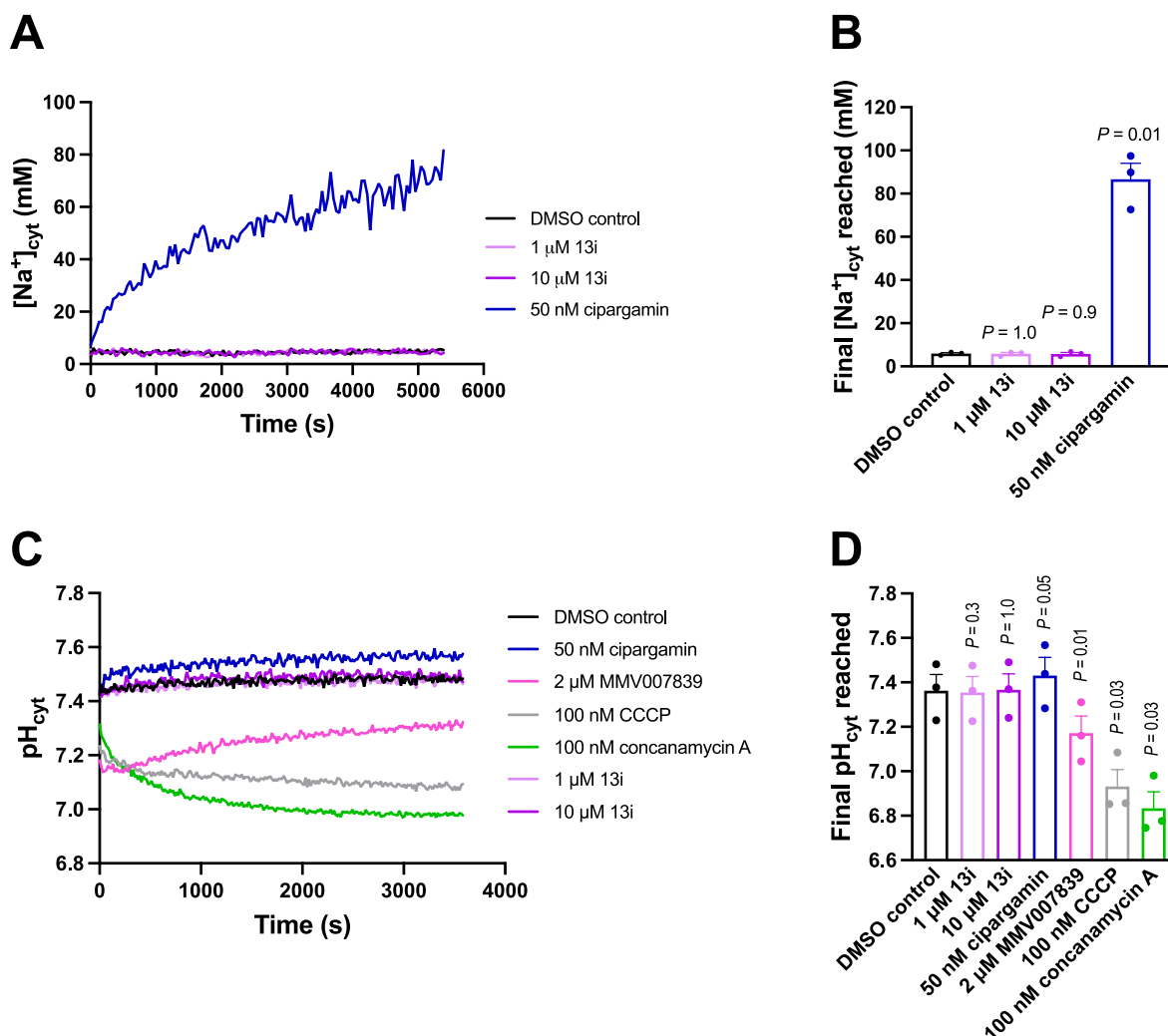
Fig. 3. Compound 13i does not affect parasite [Na^+]_{cyt} or pH_{cyt} . (A,B) Isolated 3D7 parasites loaded with SBFI were exposed to 13i (purple; 1 \mu M or 10 \mu M ), solvent alone (black; DMSO control), or cipargamin (blue; 50 nM; positive control for Pf ATP4 inhibition). (C,D) BCECF-loaded 3D7 trophozoites were exposed to 13i (purple; 1 \mu M or 10 \mu M ), cipargamin (blue; 50 nM; positive control for Pf ATP4 inhibition), MMV007839 (pink; 2 \mu M ; positive control for Pf FNT inhibition), CCCP (grey; 100 nM; protonophore), concanamycin A (green; 100 nM; positive control for V-type H^+ -ATPase inhibition) or solvent alone (black; DMSO control). Panels A and C show representative traces from a single Na^+ (A) or pH (C) experiment. Panels B and D show data averaged from three independent experiments performed on different days in which all compounds/concentrations were tested concurrently. The bars and error bars show the mean + SEM and the symbols show the data from each individual experiment. The data for each compound and concentration were compared to those for the DMSO control using one-way ANOVA with Dunnett's multiple comparisons test, with the p values shown on the figure. The final [Na^+]_{cyt} (B) and pH_{cyt} (D) reached were averaged from the data points obtained 85–90 min and 55–60 min after parasites were first exposed to the compound/solvent, respectively. The DMSO concentration was 0.1% v/v in pH experiments and 0.1–0.2% v/v in Na^+ experiments.
